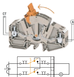
Switching the lever link
