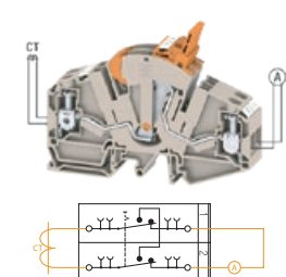
Wiring of current transformer and ammeter
