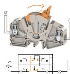
Restoring the lever link back into original position
