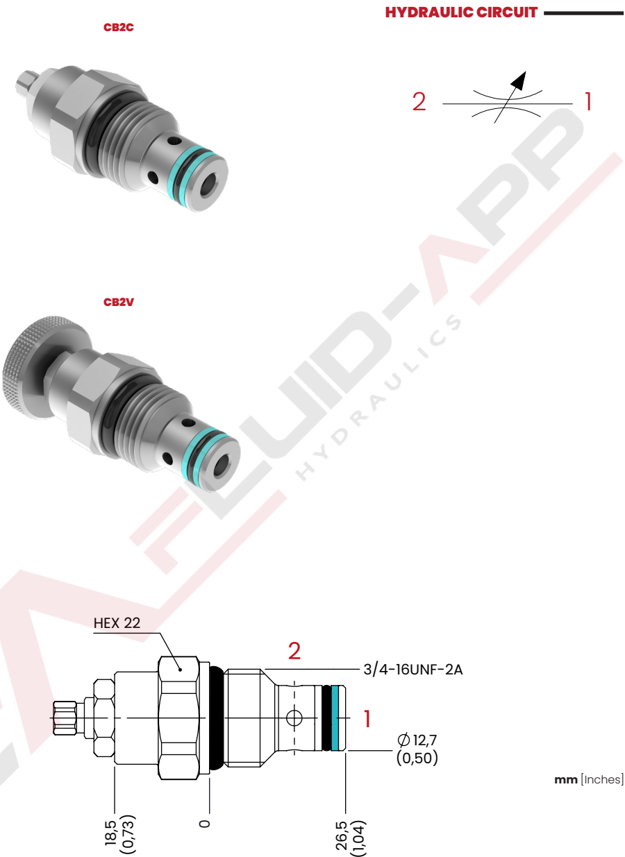
HYDRAULIC CIRCUIT
